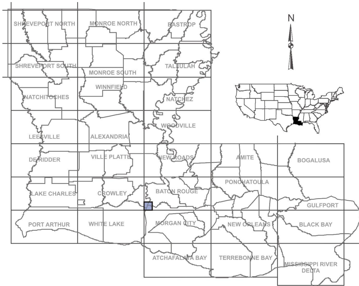
1. Location of Youngville 7.5-minute quadrangle, southeastern Louisiana.
